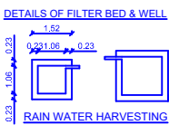
RAIN WATER HARVESTING
