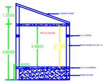
SECTION ON "AA"
