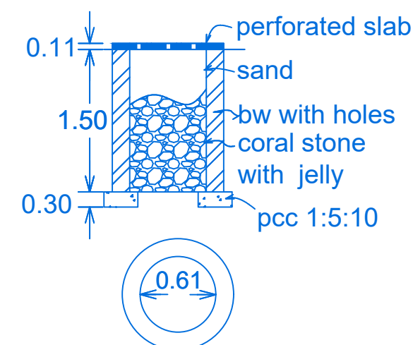
PERCOLATION PIT
