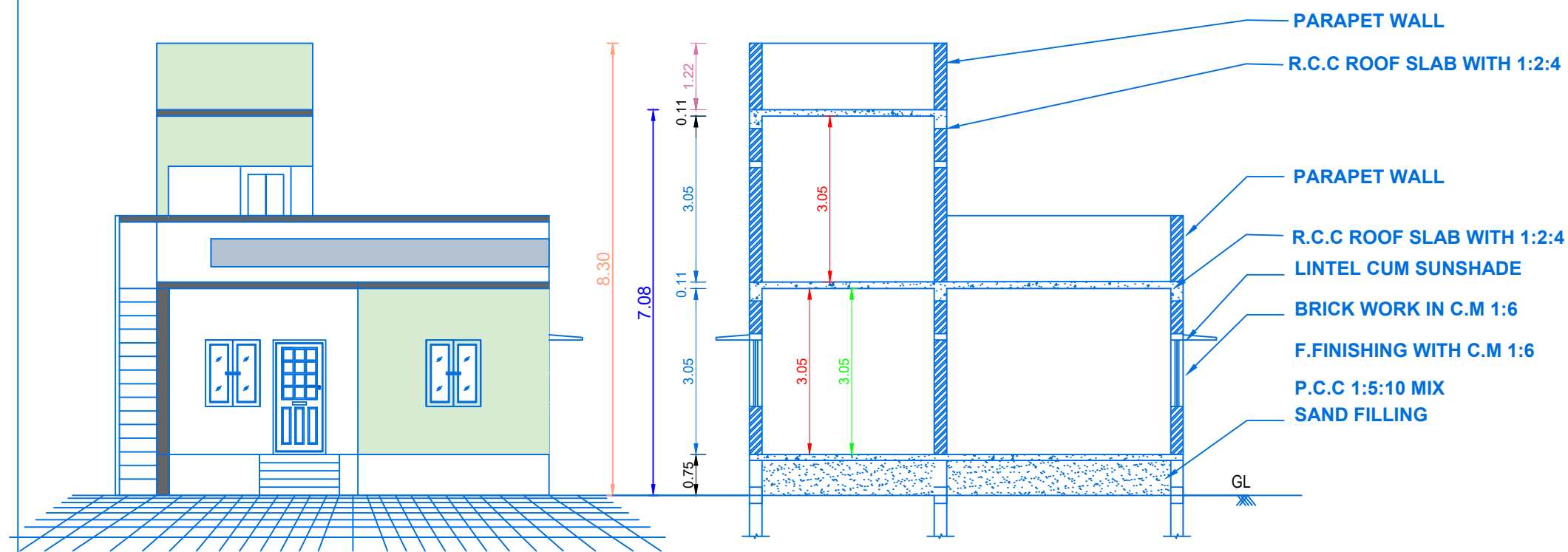
FRONT ELEVATION
