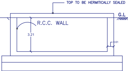
RWH SECTION (SAMPLE) RWH_CAPACITY_L=2000LTRS
