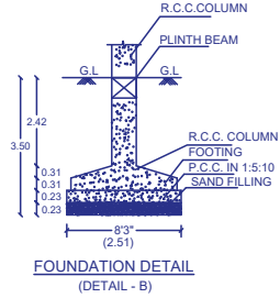
FOUNDATION DETAIL (DETAIL - B)
