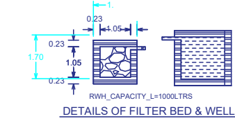
DETAILS OF FILTER BED & WELL
