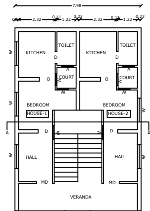
PRO S.FLOOR PLAN
