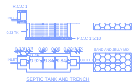
SEPTIC TANK AND TRENCH
