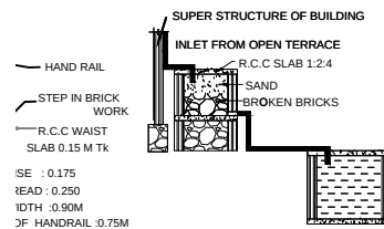
RAINWATER HARVESTING
