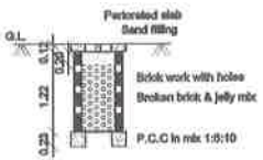
PERCOLATION PIT FOR 30 Sq. m. (Scale: 1:50)
