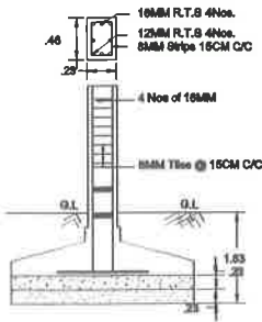
RCC COLUMN DETAILS
