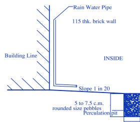
PERCOLATION PIT
