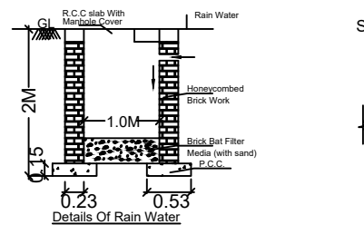
Collection Pit (Recharge Well Method) SCALE:- 1"=4'0"
