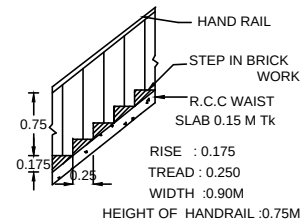
STAIR DETAILS
