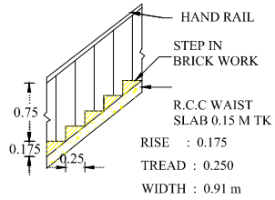
STAIR DETAILS
