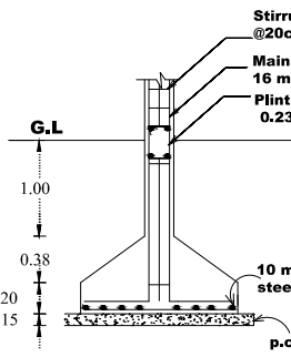
Details of column footing
