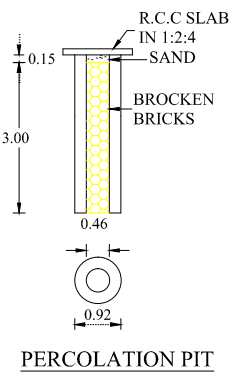
PERCOLATION PIT
