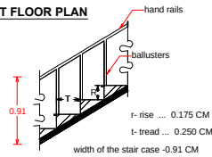
Details of staircase
