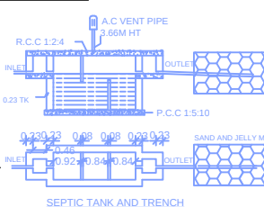
SEPTIC TANK AND TRENCH
