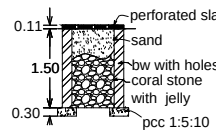
percolation pit
