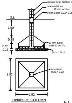
Details of COLUMN
