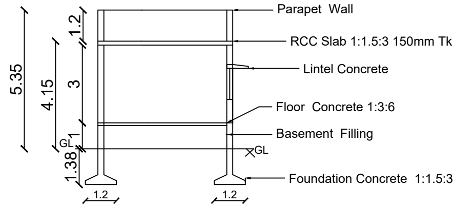
SECTION A - A VIEW
