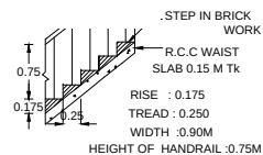
STAIR DETAILS
