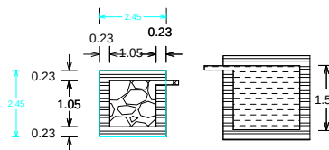
DETAILS OF FILTER BED & WELL
