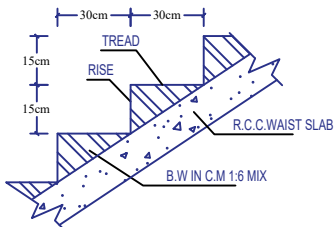
STAIRCASE DETAILS
