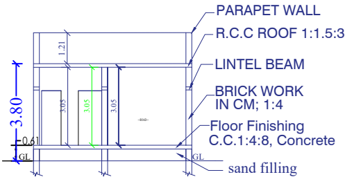
SECTION NN
