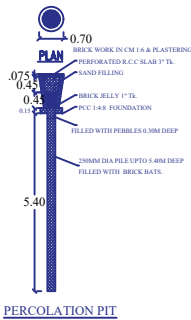
PERCOLATION PIT
