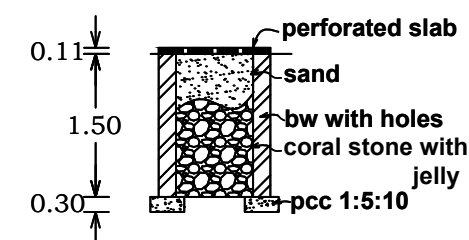
Percolation pit
