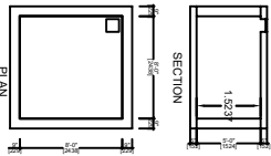
DETAILS OF COLLECTION SUMP FOR RAIN WATER HARVESTING OF ROOF TOP RAIN WATER RWHT_CAPACITY_L=5000LITRS
