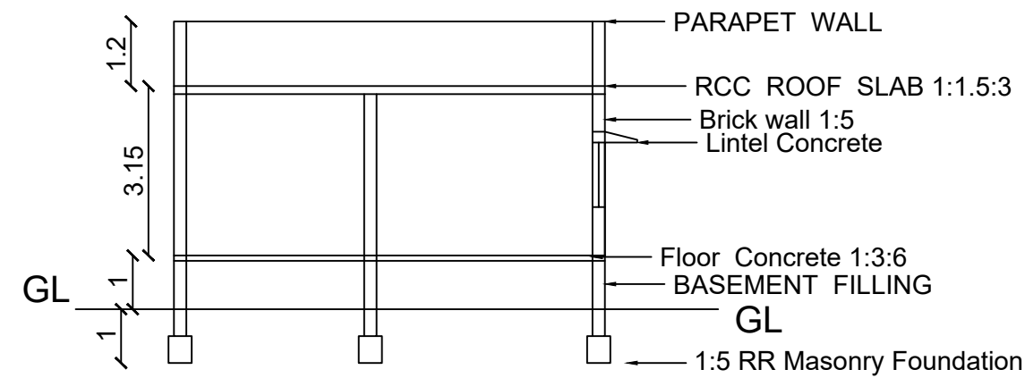
SECTION A-A VIEW
