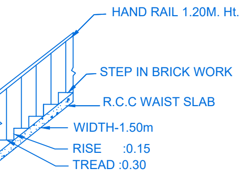
STAIR DETAIL
