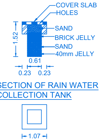
PLAN
