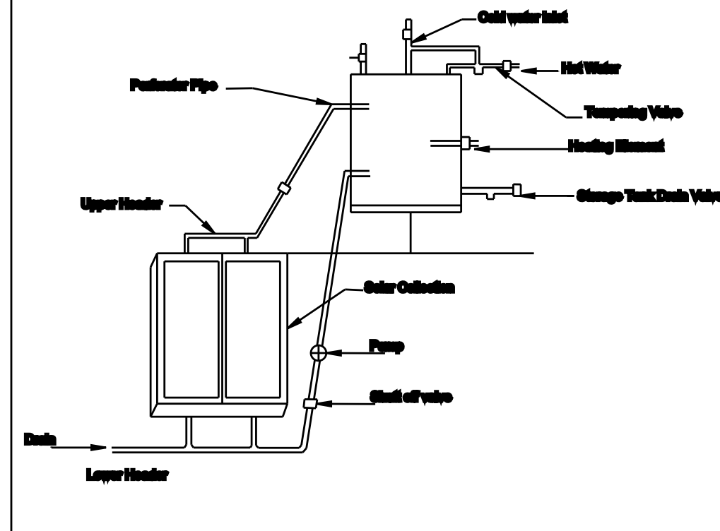
Details Of Solar Water Heater (NTS)
