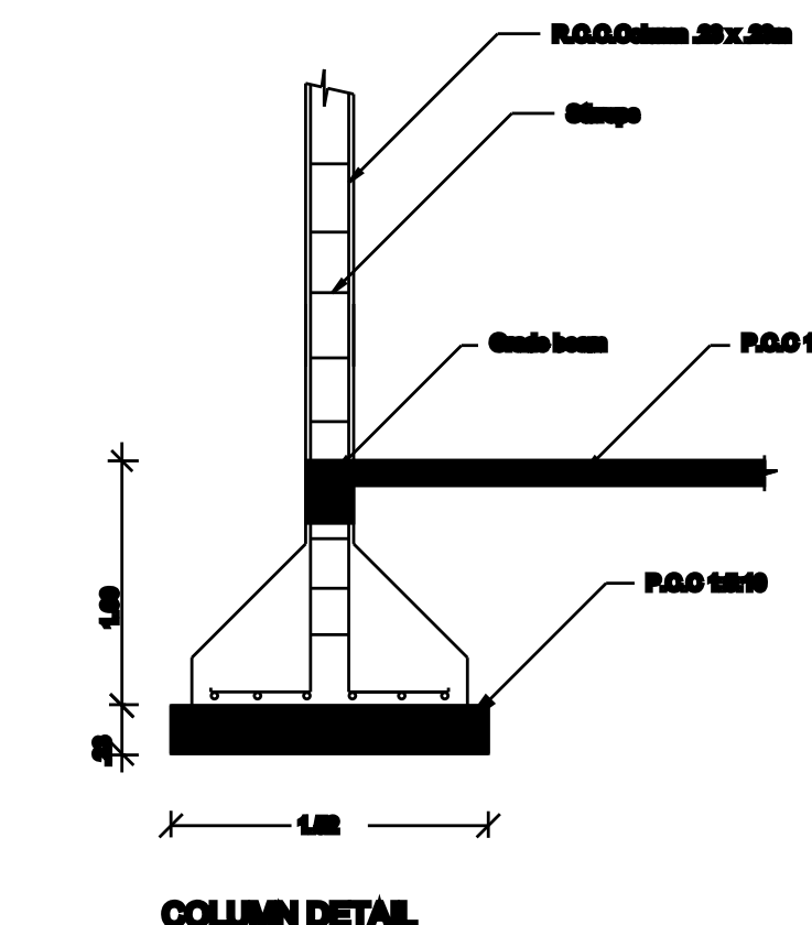
COLUMN DETAIL
