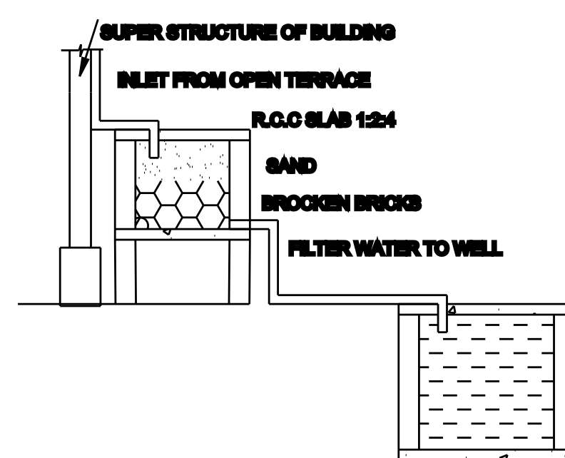
RAINWATER HARVESTING
