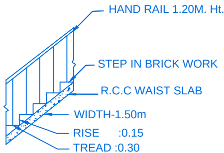
STAIR DETAIL
