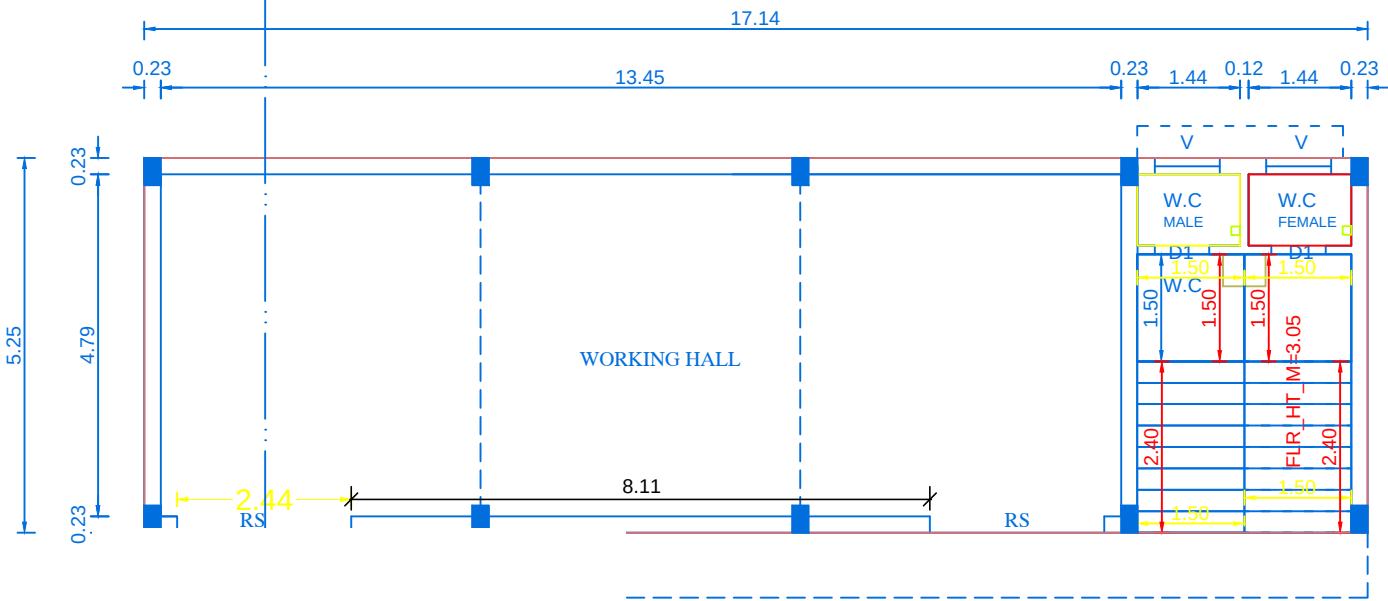
2D FLOOR PLAN (BLOCK-2)
