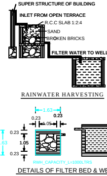
DETAILS OF FILTER BED & WELL
