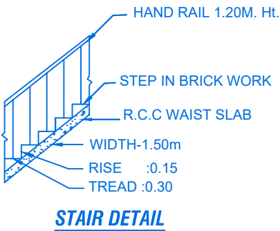
STAIR DETAIL
