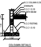
COLUMN DETAILS
