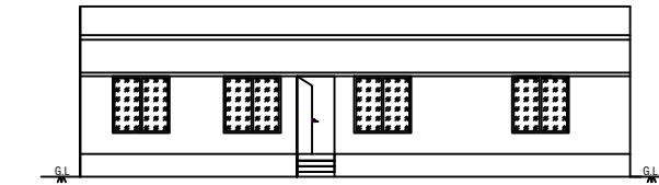
FRONT ELEVATION
