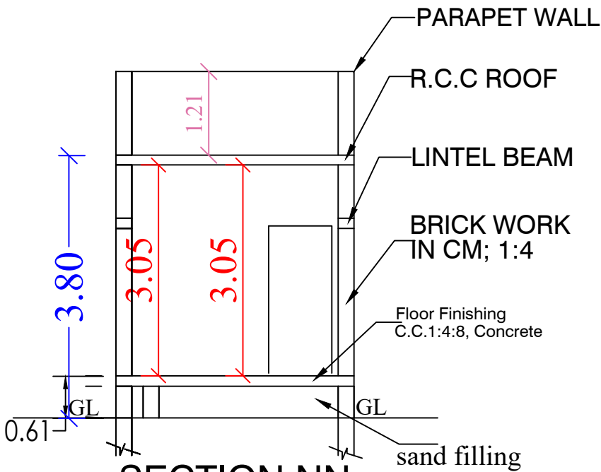
SECTION NN
