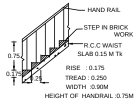
STAIR DETAILS
