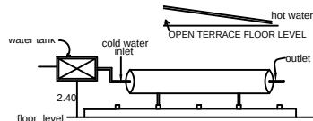
Details of solar water heating system
