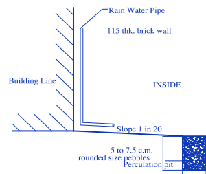
PERCOLATION PIT
