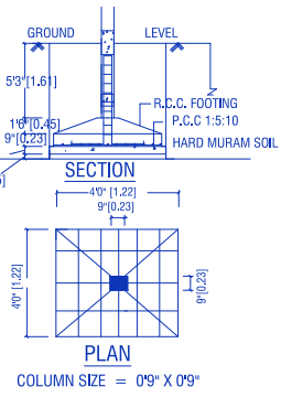
FOUNDATION DETAILS
