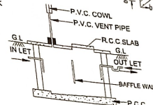
SEC. OF SEPTIC TANK
