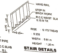
STAIR DETAILS
