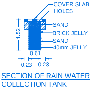
SECTION OF RAIN WATER COLLECTION TANK PLAN
