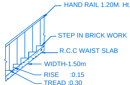
STAIR DETAIL
