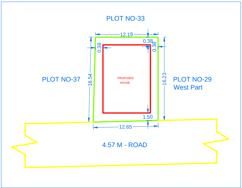
LOCATION PLAN Scale 1:400
