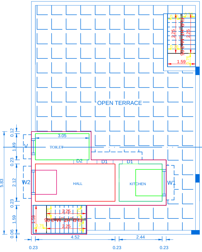
PROP.SECOND FLOOR PLAN
