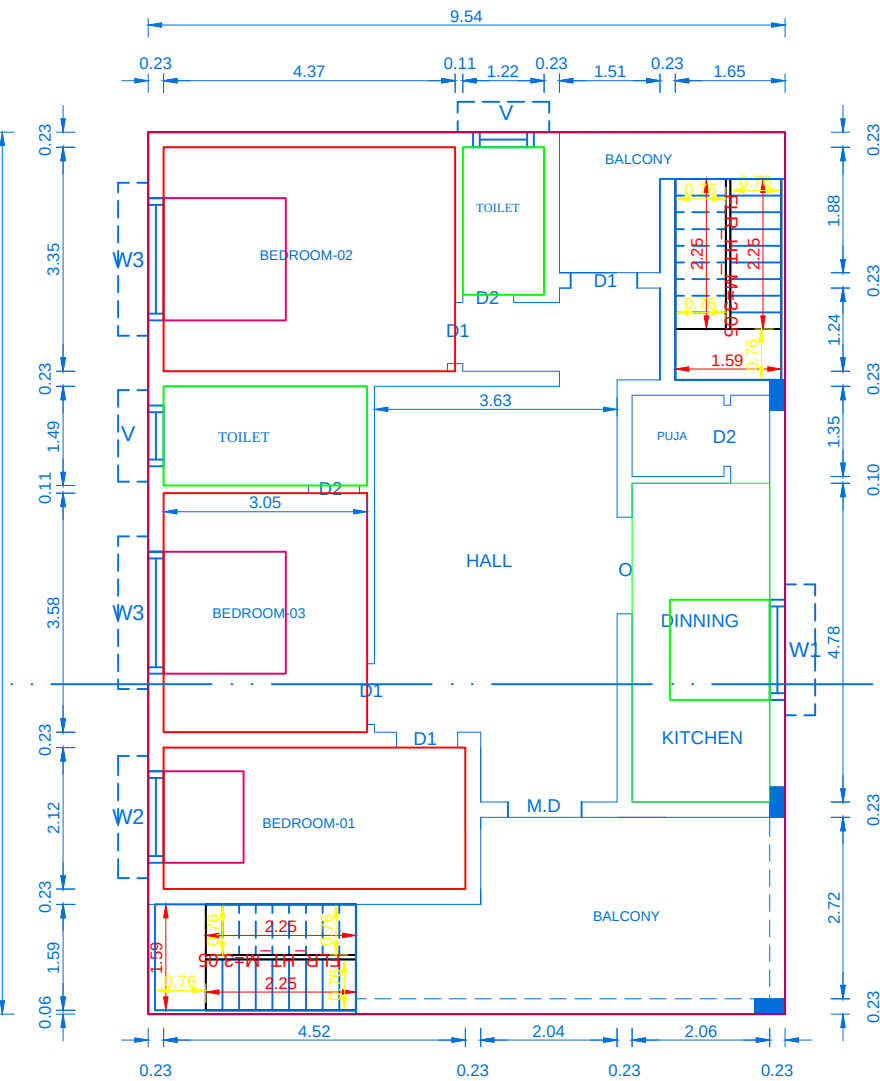
PROP.FIRST FLOOR PLAN
