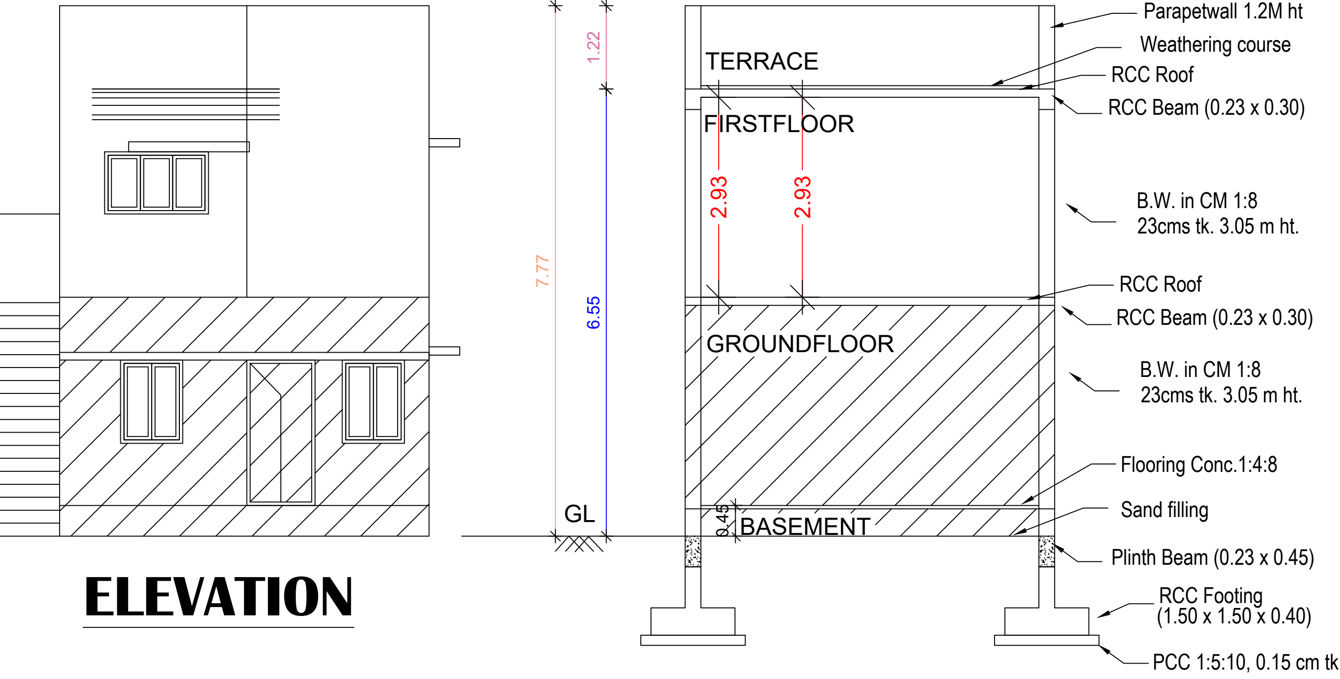
SECTION - "AA"
