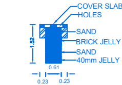
SECTION OF RAIN WATER COLLECTION TANK
