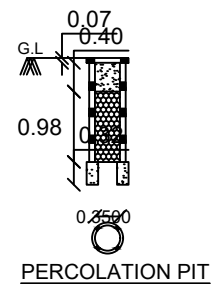
PERCOLATION PIT
