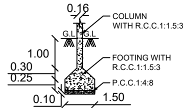
COLUMN WITH FOOTING DETAIL
