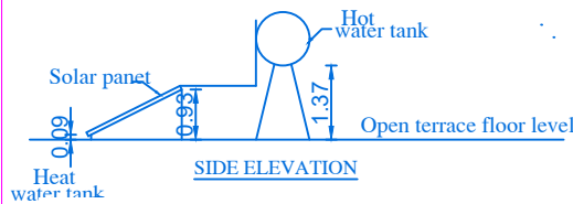
SIDE ELEVATION
