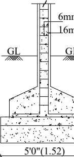
COLUMN FOUNT
