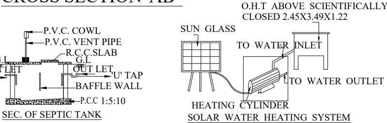
CROSS SECTION"AB"
