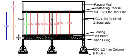
SECTION AB
