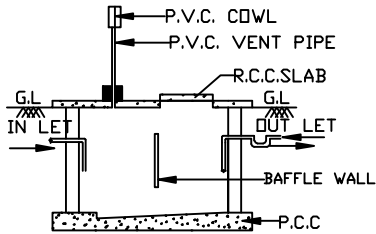
SEC. OF SEPTIC TANK
