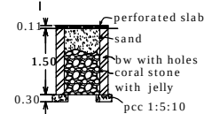
percolation pit
