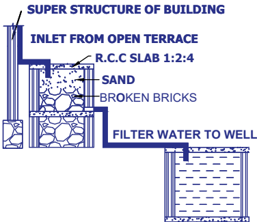
RAINWATER HARVESTING
