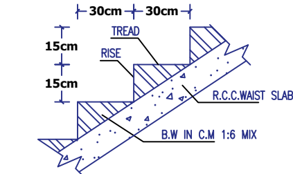
STAIRCASE DETAILS
