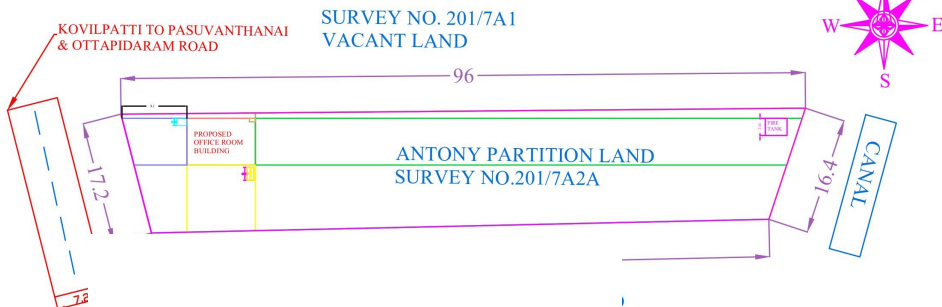
PLAN LAYOUT
