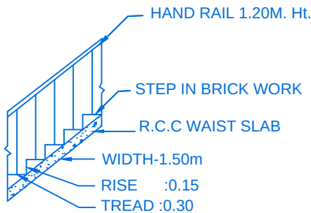
STAIR DETAIL
