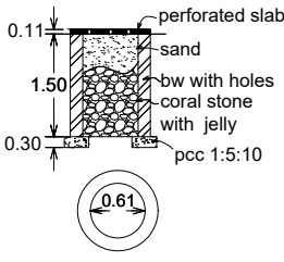
percolation pit
