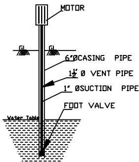
SEC. OF BOREWELL
