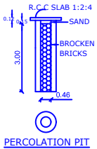
PERCOLATION PIT
