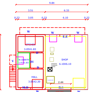
HOUSE SHOP GROUND FLOOR PLAN
