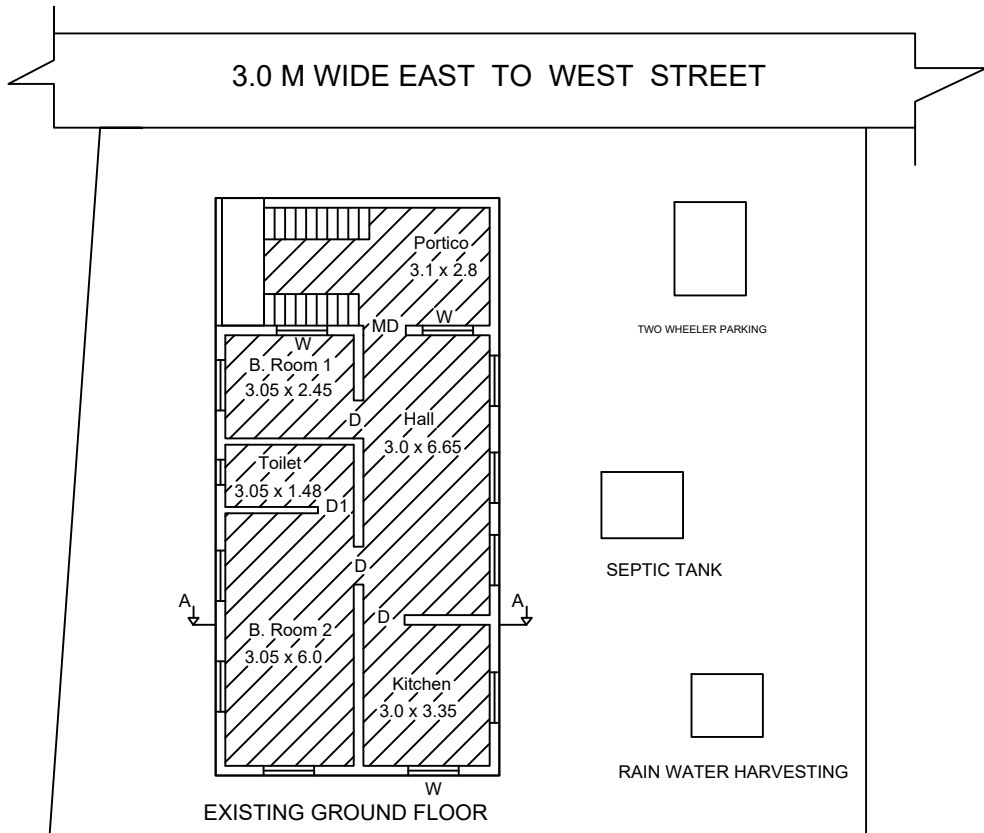
SITE CUM GROUND FLOOR PLAN
