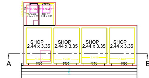
Pro. Ground Floor
