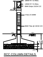
RCC COLUMN DETAILS
