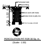
PERCOLATION PIT FOR 30 Sq. m. (Scale: 1:50)
