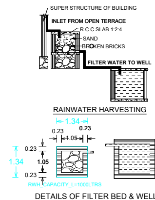
DETAILS OF FILTER BED & WELL
