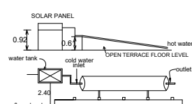
Details of solar water heating system
