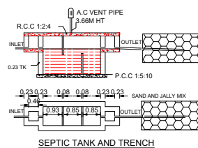
SEPTIC TANK AND TRENCH
