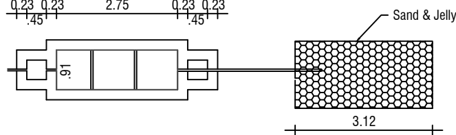
SEPTIC TANK & TRENCH
