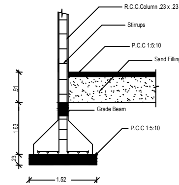
COLUMN DETAIL
