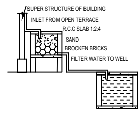
RAINWATER HARVESTING
